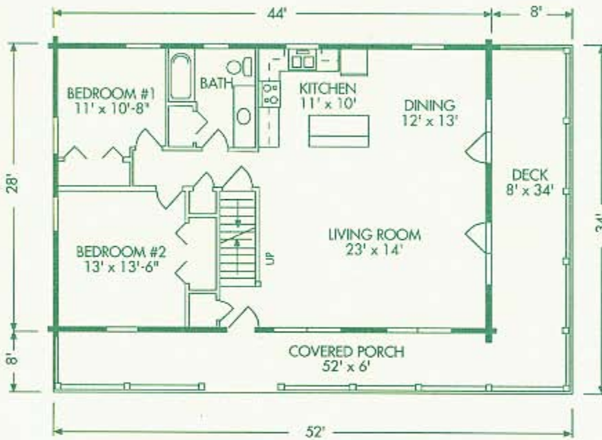
MAIN FLOOR
