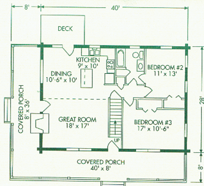
MAIN FLOOR
